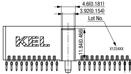
Contact Dimension
