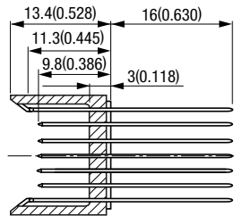
X-X' Cross Section
