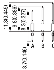
Contact Dimension
