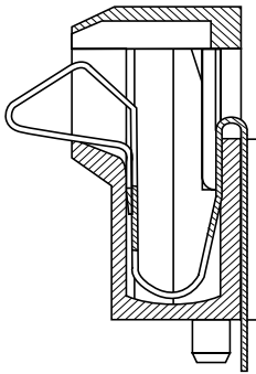
X-X' Cross Section
