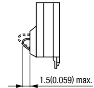
Effective contact displacement range
