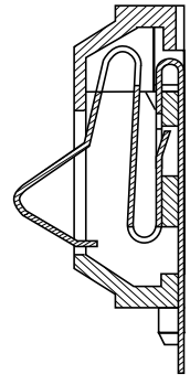
X-X' Cross Section
